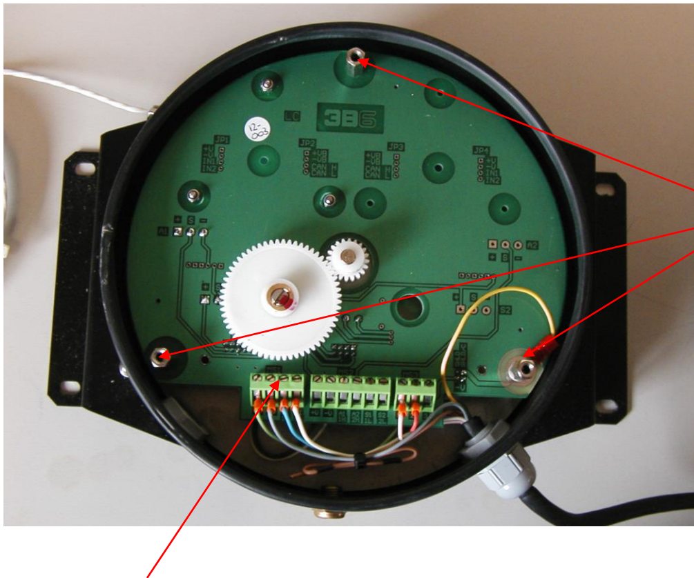
MS1/A1 Angle output
